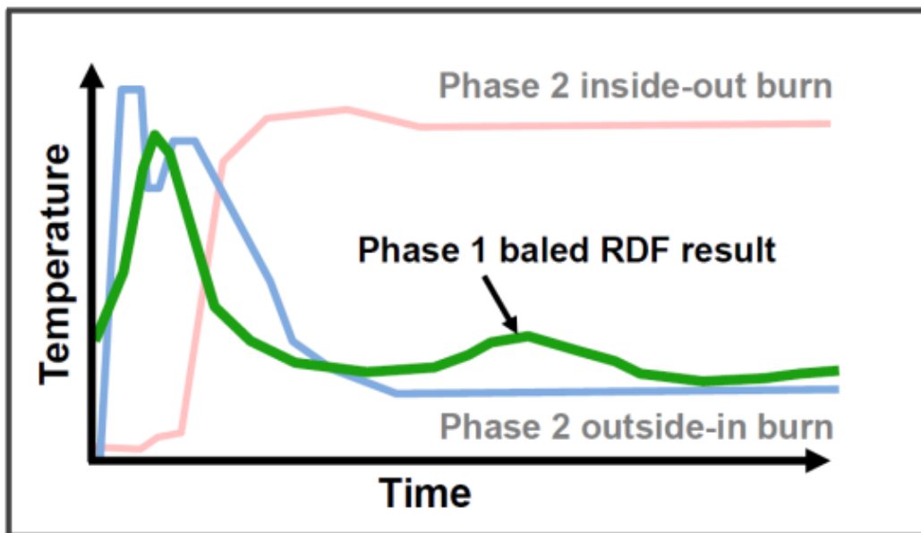
Graph 5: Illustrative outside-in and inside-out burn temperatures compared with an example smaller scale baled waste test result
