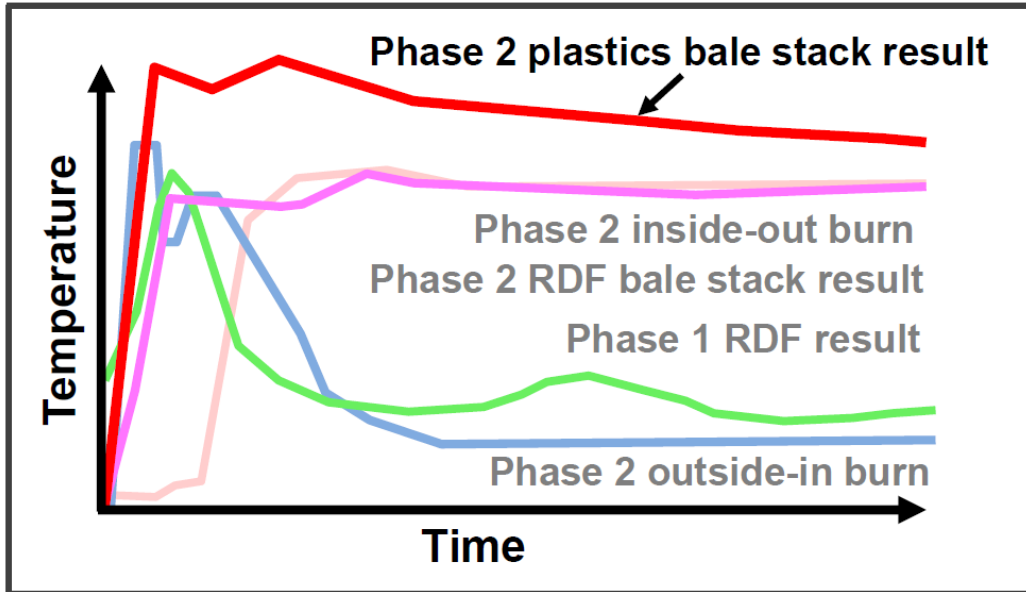
Graph 7: Illustrative comparison between plastics and other typical other wastes during bale stack burn tests
