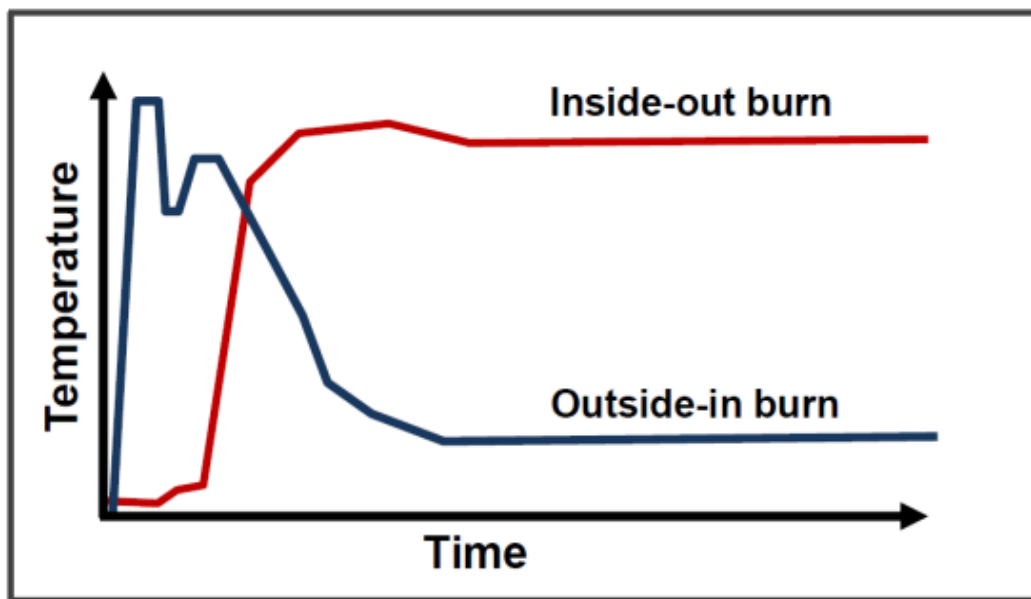
Graph 4: Illustrative loose waste stack outside-in and inside-out burn temperatures
